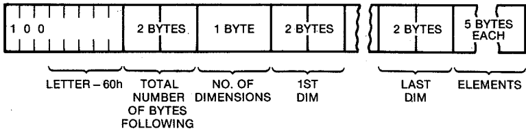
Fig. 3-5. Data structure for numeric array.
